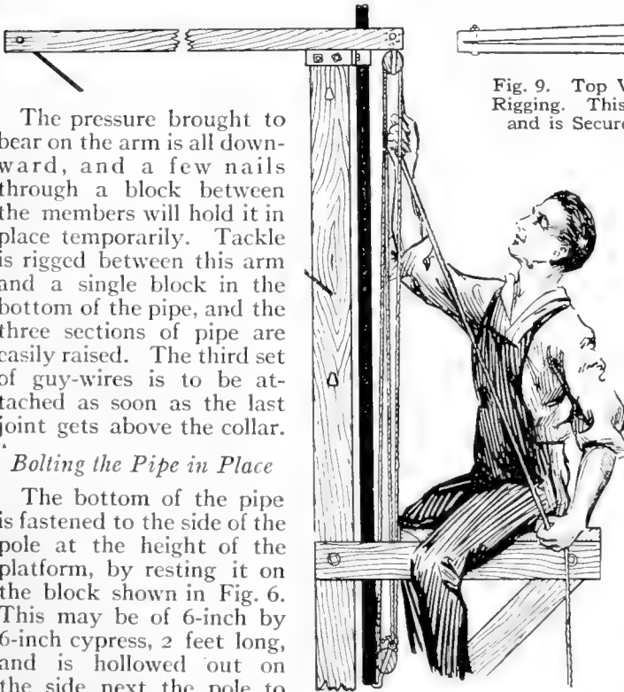
Fig. 8. Showing Rigging of Temporary Arm for Final Lift
